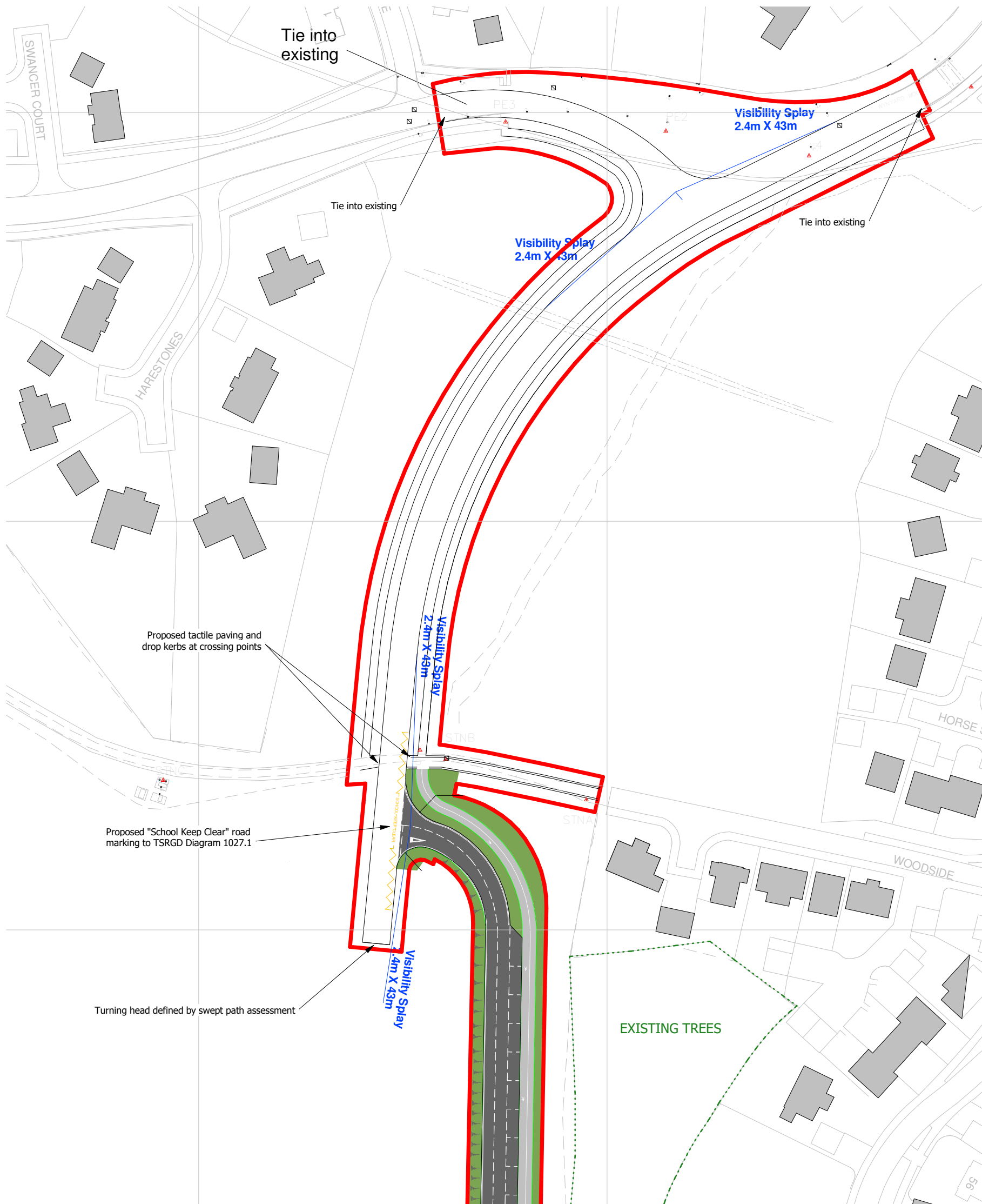
Proposed Site Plan 1 : 500
